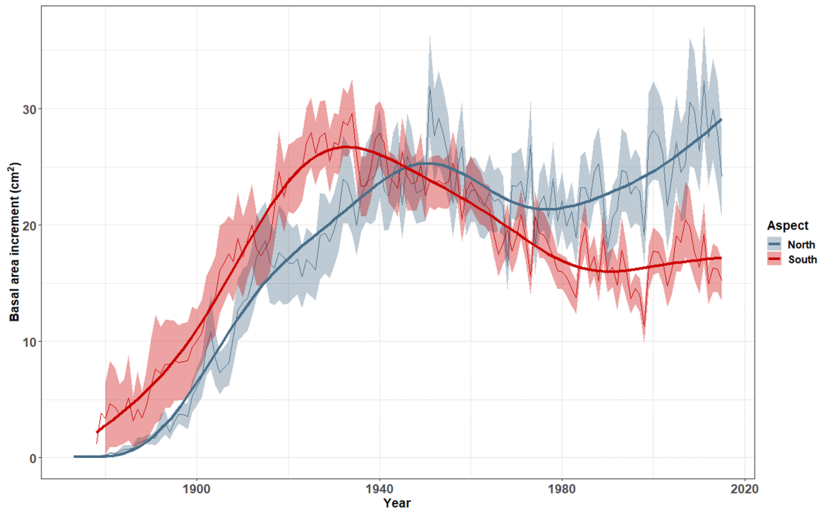
Fig. 2. Reversal of growth patterns between trees growing on contrasting topographic aspects. Growth trends are measured as BAI. Thin lines are mean values, and shaded areas represent SEs. Thick lines are fitted curves from a general additive model using “year” and “aspect” as smoothing terms.
